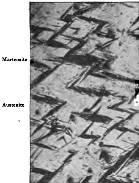
Fig. 63. Martensite (black) in Austenite (white). Steel of about 1.50 per cent Carbon. Quenched at 1,050^{\circ} C. in ice water. (Osmond, The Metallographist , II, p. 261, et seq. )
